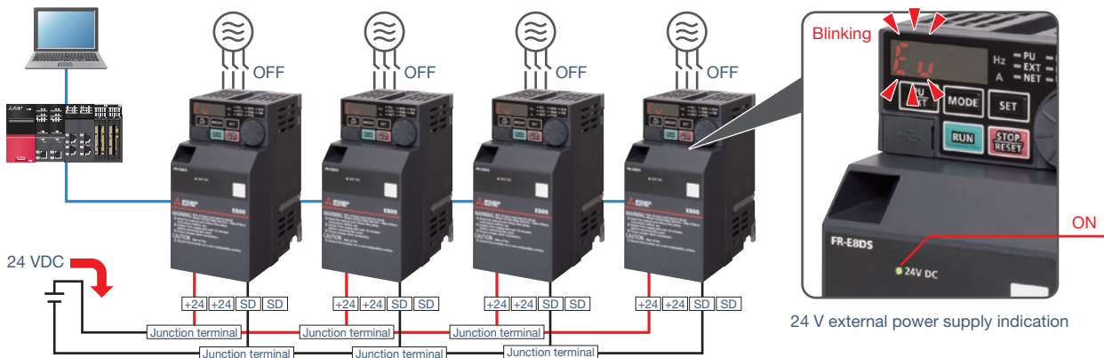
Up to four inverters can be connected in series.
